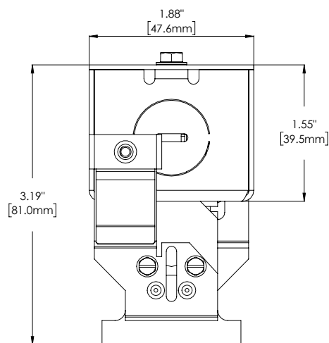
15/16" GEMINI Single Lens GEM1-XX-X-24-XX-X-W-UNV
