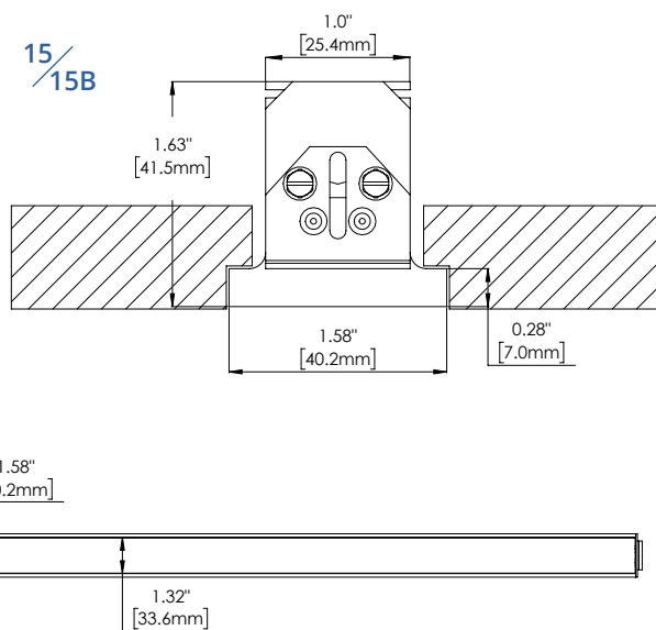
9/16" GEMINI Single Lens GEM1-XX-X-15/15B-XX-X-W-UNV
