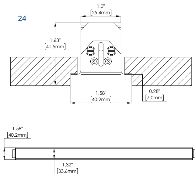
15/16" GEMINI Single Lens GEM1-XX-X-24-XX-X-W-UNV
