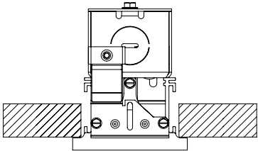
LAY-IN TILE INSTALLATION
