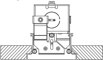
TEGULAR TILE INSTALLATION
