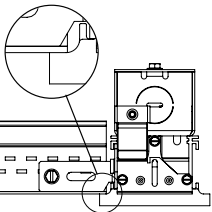
9/16" OR 15/16" FLAT GRID
