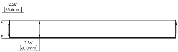
9/16" GEMINI Single Lens GEM2-XX-X-X-15/15B-XX-X-W-UNV
