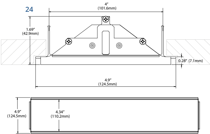
15/16" GEMINI Single Lens GEMS-XX-X-X-24-XX-X-W-UNV
