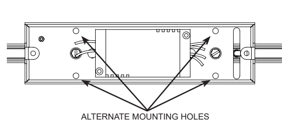
ALTERNATE MOUNTING HOLES
