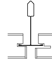
15/16" Flat Grid w/ Partially Concealed Tiles
