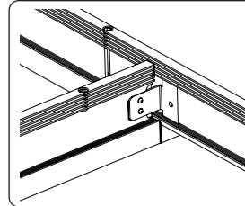
DETAIL E ALIGNING BRACKET WITH HOLE
